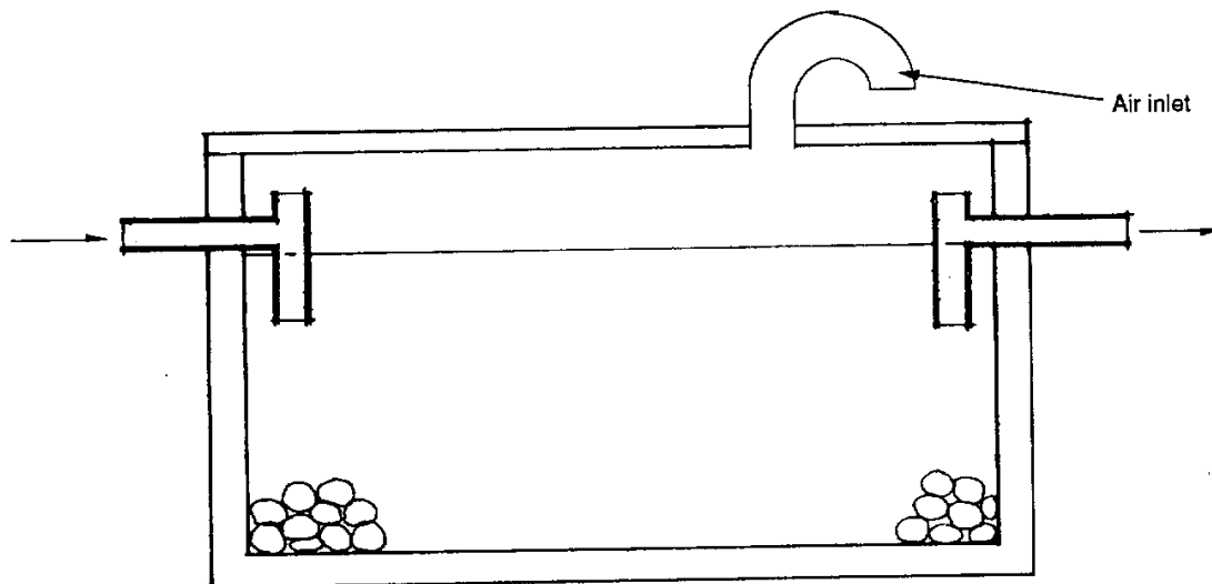
FIGURE 3.5 AEROBIC FILTER
