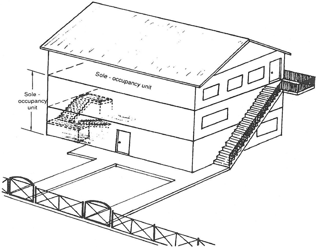
Sketch A3.2 (d) (ii) Example of a Class 1 Building – Two Sole-Occupancy Units Each with Independent Direct Egress to a Road or Open Space.
