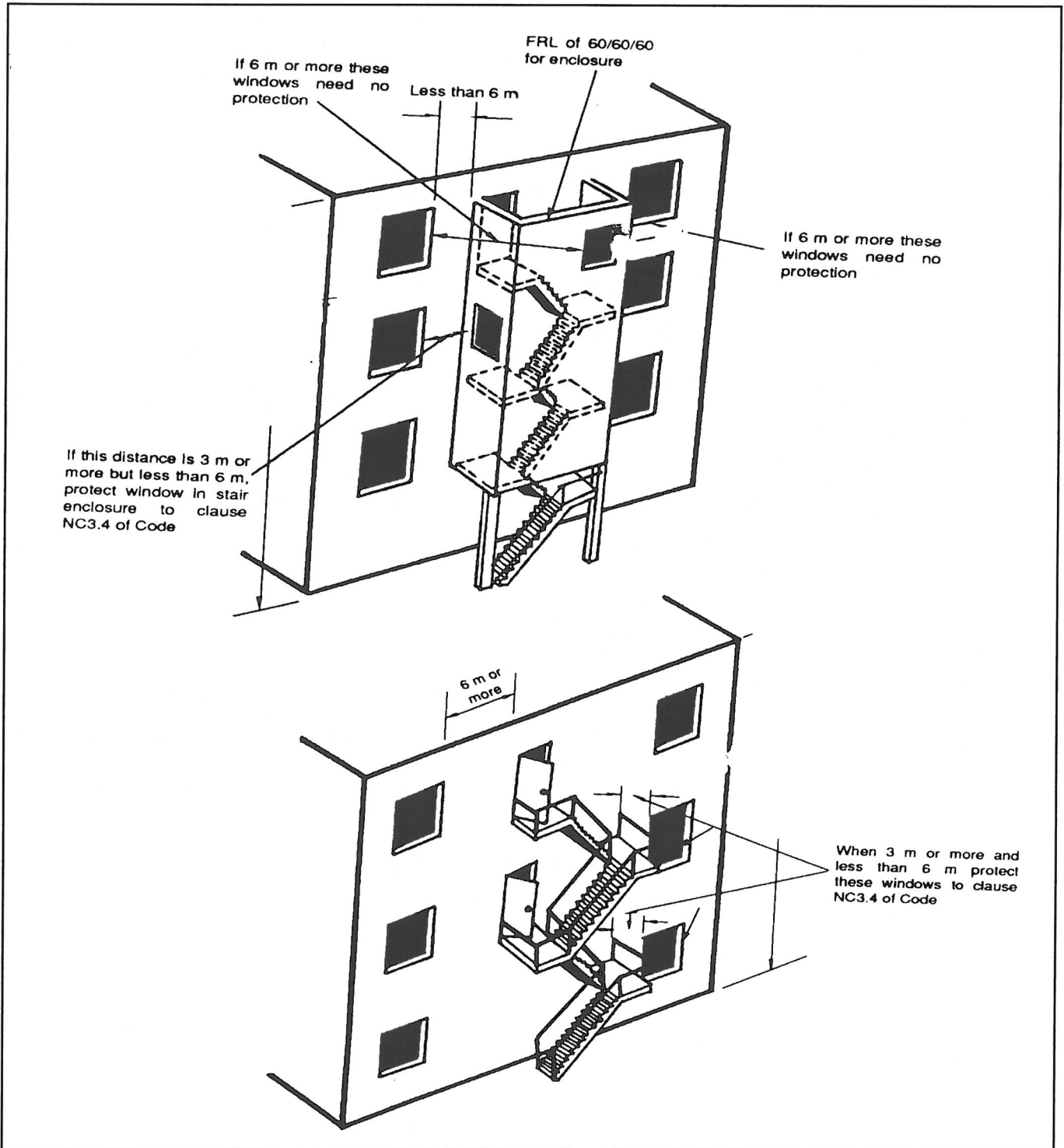
Sketch ND1.8 Requirements for External Stairways
