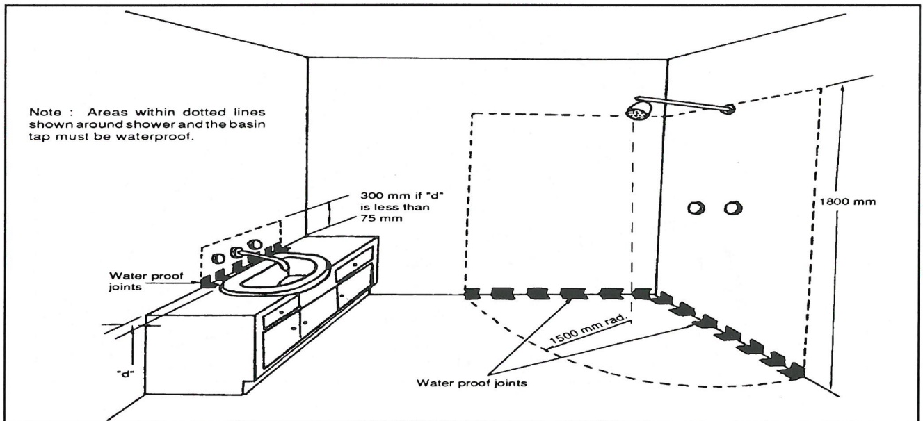
Sketch DF1.6 Requirement for Water Proofing of Areas Around Showers, Basins, Sinks, etc.
