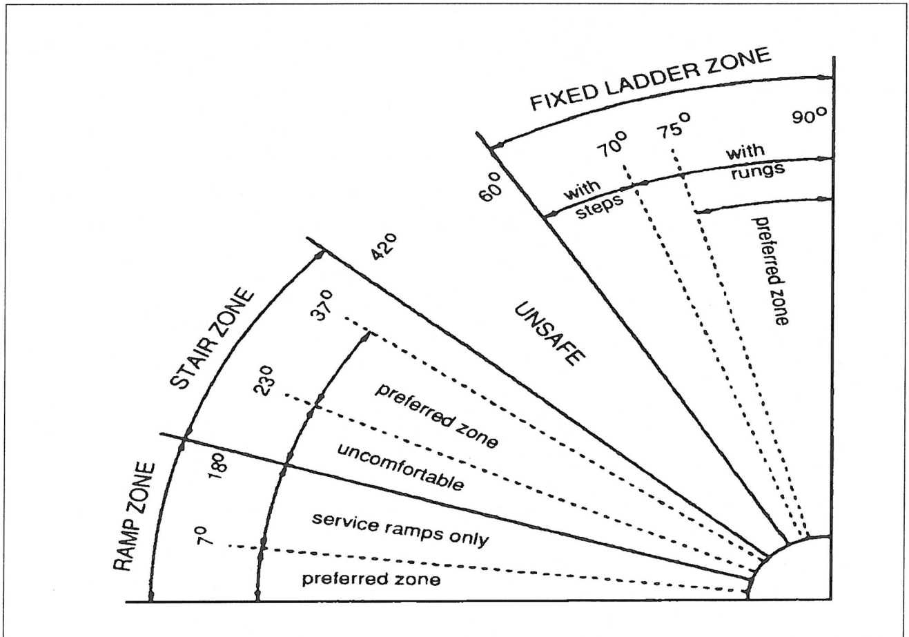
Sketch DD1.1 Recommended Pitch for Ramps, Stairs and Ladders
