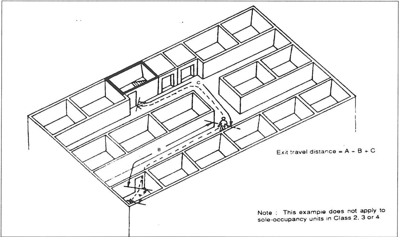
Sketch ND1.15 (i) Example of the Measurement of Distance from any point on a floor to a Single Exit
