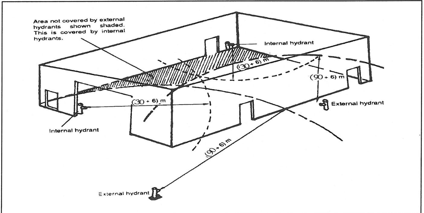
Sketch NE1.4 Arrangement of External and Internal Hydrants to cover Total Area
