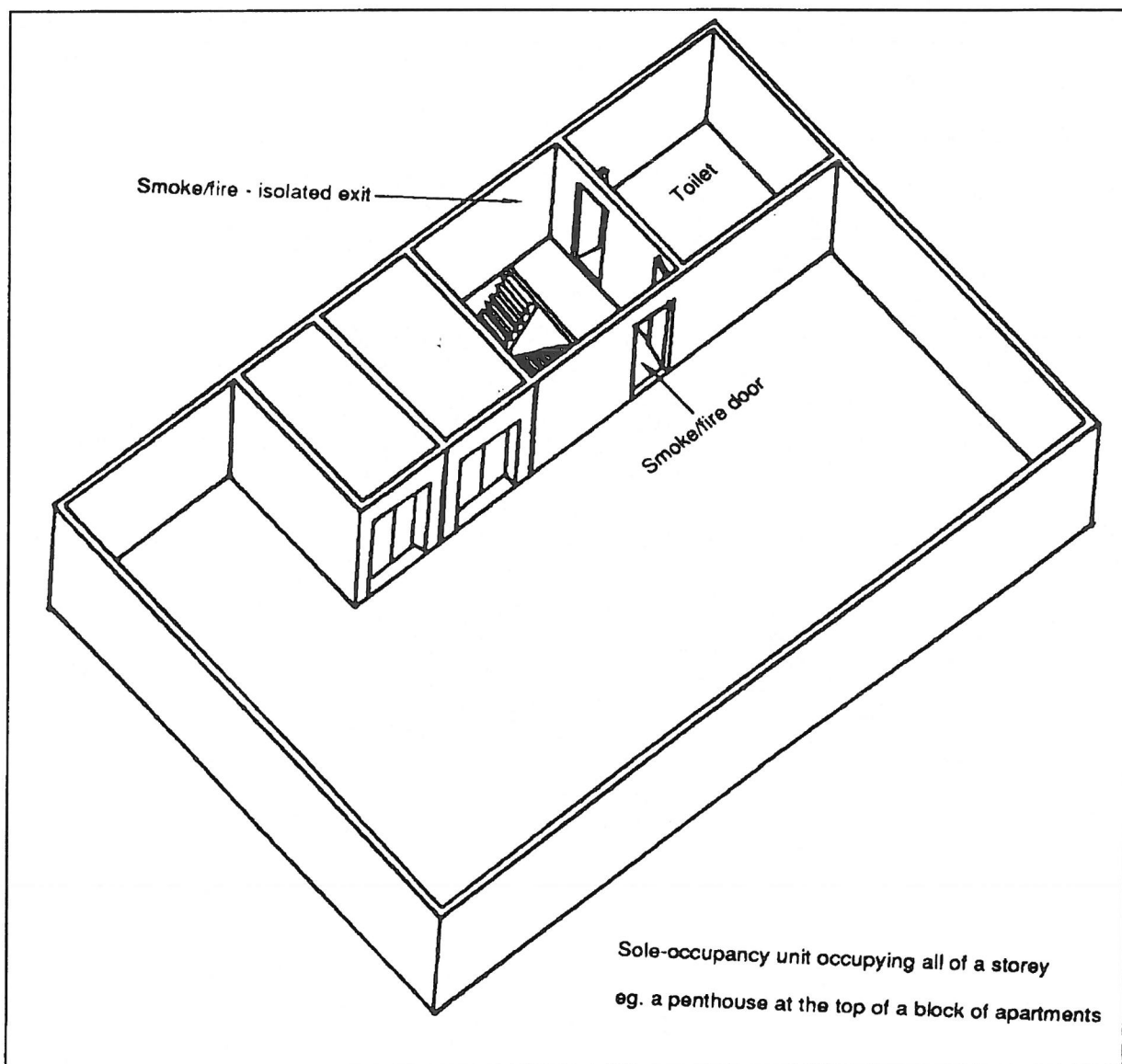
Sketch ND1.7 (a) (ii) Example of Doorways Permitted to Open Directly from a Room to a Smoke or Fire-Isolated Exit
