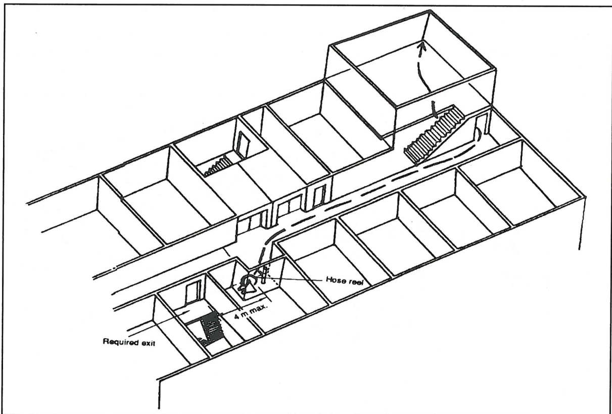
Sketch NE1.5 Arrangement of Hose Reel and the Reach of the Hose to the Farthest Point on the Floor
