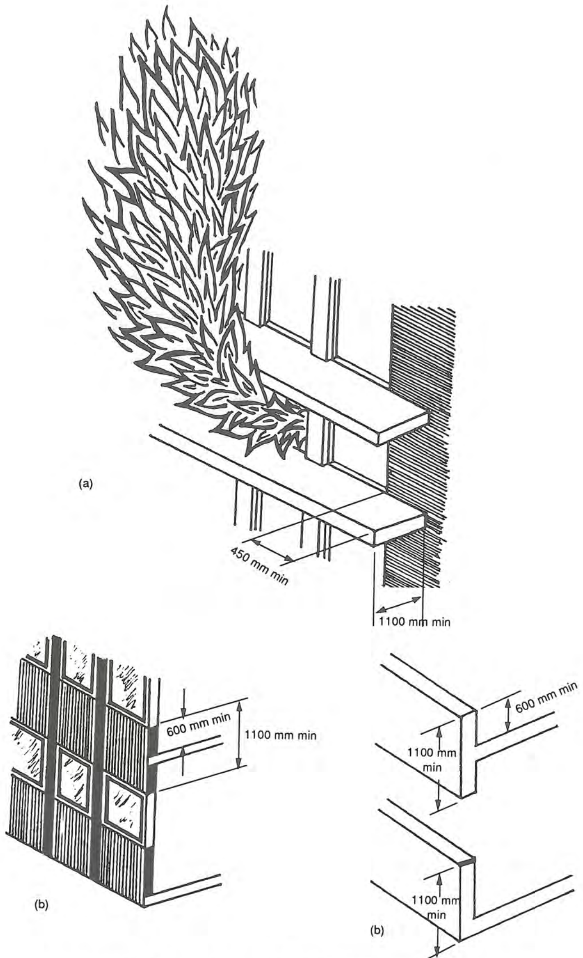
Sketch NC2.6(b) Protection of Openings With Horizontal Projections or Spandrel Walls
