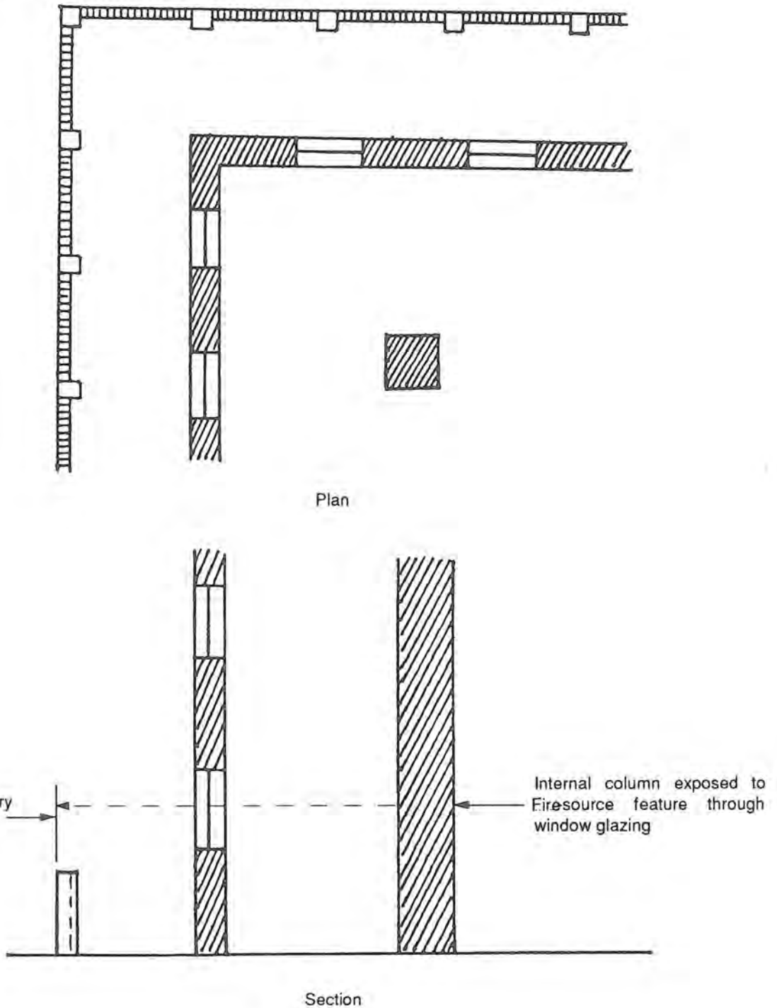
Sketch Spec NC1.1 (i) Exposure to Fire-Source Feature
