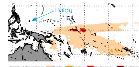
Figure I7d. 4-week coral bleaching outlook for Palau (Coral Reef Watch, 03/07/2019). Figure modified from NOAA (2019).
