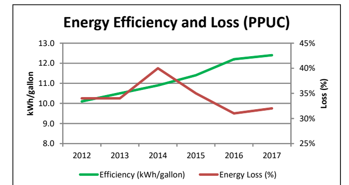
Figure I110a. Energy efficiency and losses. Data from PPUC (2017).
