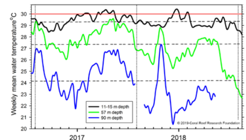
Figure I7c. The two year trends of weekly water temperature show how at times the water column is nearly the same temperature from the surface to 90 m depth (March-April 2018) and can quickly switch to highly stratified temperatures (May 2018). The past two years (2017-2018) have had only short periods of near surface temperatures above the nominal 30° C coral bleaching threshold. Such short excursions above that level do not usually induce bleaching unless they persist for some weeks. Figure from Colin (2018).
