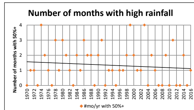
Figure I11c. Orange dots indicate the number of months in that year with higher-than-average rainfall. This graph compares monthly totals to the monthly average (e.g. each January total is compared to the January 1970-2016 average), and shows the number of months per year where the monthly total was 50% or greater than the average monthly rainfall.
