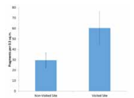
Figure I14. Density of coral fragments at visited and non-visited sites in the Rock Islands. Figure from Nester et al. (2017).
